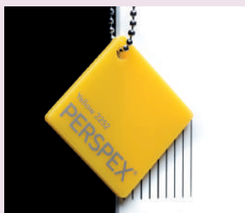
Colour: Yellow Code: 2252 Dimensions(mm): 3050 x 2030 Thickness (mm): 3, 5 Light Transmission (%): 21
