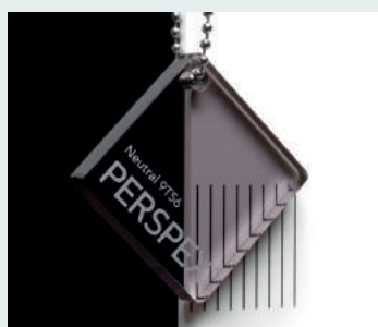
Colour: Neutral Code: 9T56 Dimensions(mm): 3050 x 2030 Thickness (mm): 6, 8, 10, 12 Light Transmission (%): 46
