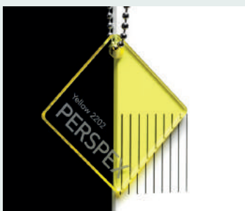
Colour: Yellow Code: 2202 Dimensions(mm): 3050 x 2030 Thickness (mm): 3, 5 Light Transmission (%): 86
