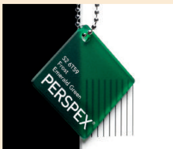
Colour: Emerald Green Code: S2 6T59 Dimensions(mm): 3050 x 2030 Thickness (mm): 3, 5 Light Transmission (%): 13
