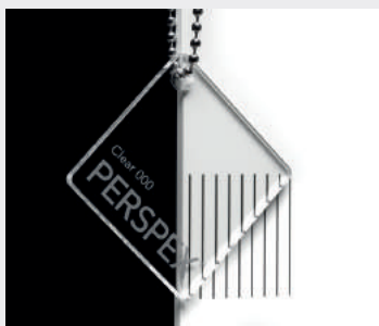
Colour: Clear Code: 000 Dimensions(mm): 3050 x 2030 Thickness (mm): 0-50 Light Transmission (%): 92
