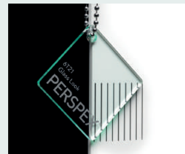
Colour: Glass-Look Code: 6T21 Dimensions(mm): 3050 x 2030 Thickness (mm): 3-10 Light Transmission (%): 90
